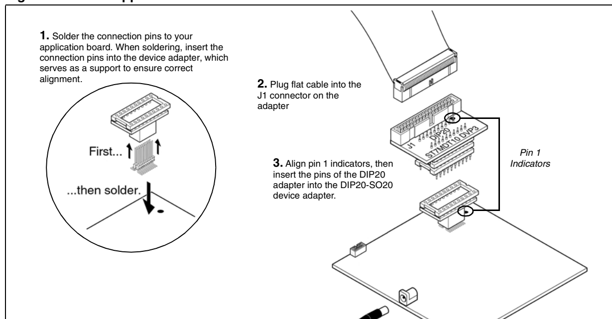
Figure 4. SO20 application board connection
